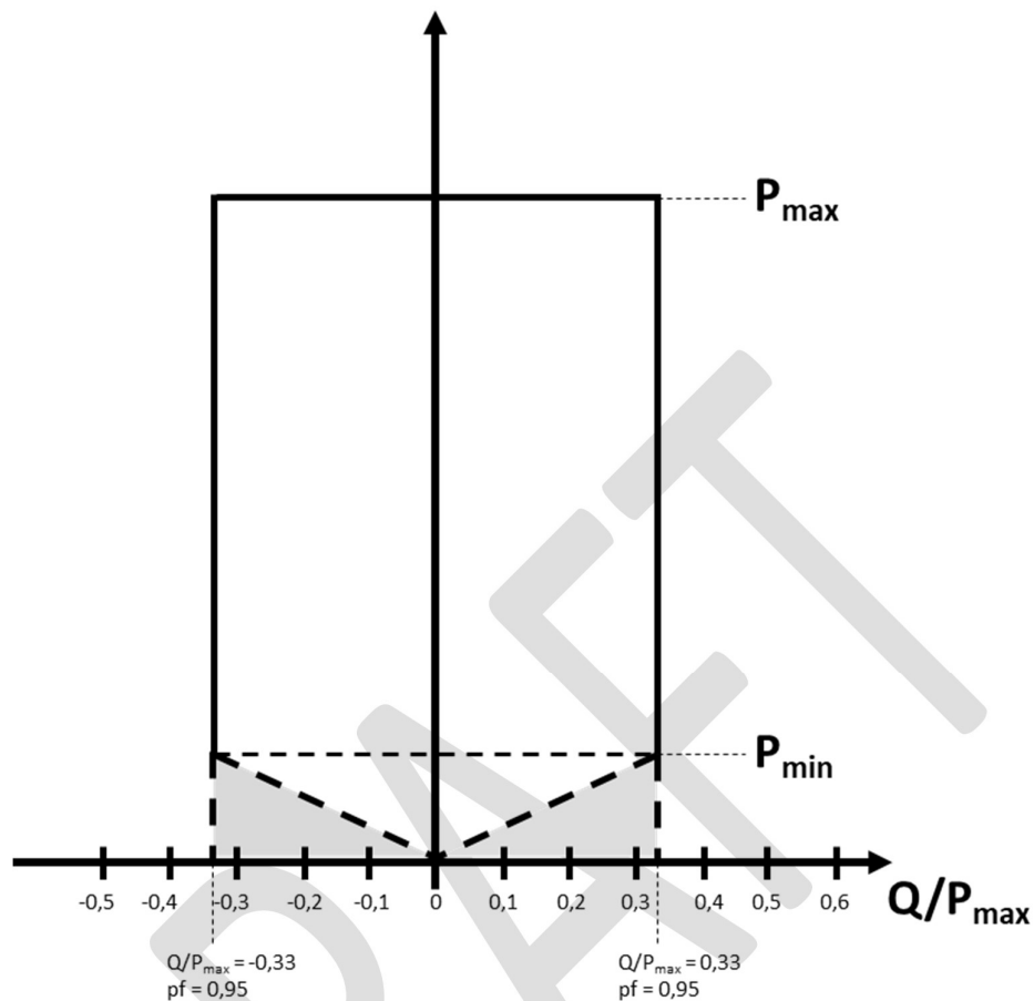
Figure 7. U-Q/Pmax-profile of a power park module. Power park modules shall be capable of operating within the envelope.
